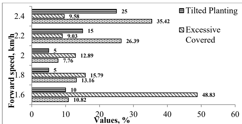
Figure 5. Tilted planting (%), excessive soil covered (%) and partially soil covered (%) observed at different speeds during evaluation of the auger conveyer type metering device
