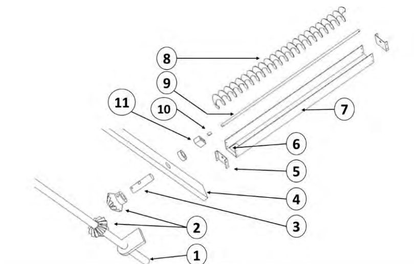
Figure 1. The isometric exploded view of the auger type metering unit
