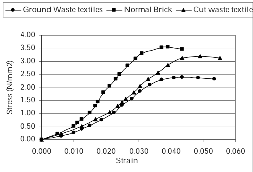
Fig. 1. Stress-strain relationships of solid cement blocks
